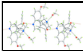
Fig. 2. Supramolecular chain in (I) mediated by O–H···N hydrogen bonds (orange dashed lines). Methanol molecules are associated with this chain via O–H···N hydrogen bonds (black dashed lines).
