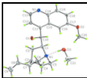
Fig. 1. Molecular structure of the asymmetric unit in (I) showing atom-labelling scheme and displacement ellipsoids at the 50% probability level. The O—H...N hydrogen bond is shown as a dashed line.
